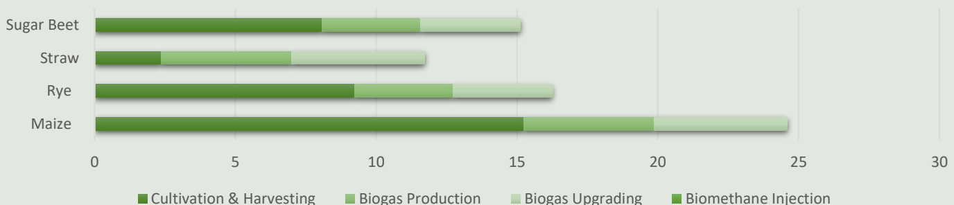
GHG Emissions per Feedstock (gCO 2 e/MJ biomethane)
